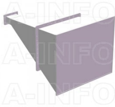
LB-430-20-ASPO Standard Gain Horn Antenna 1.7-2.6GHz 20dB Gain Rectangular Waveguide Interface
