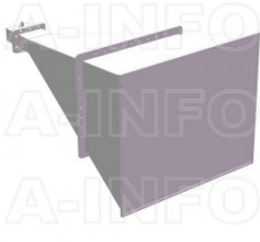
LB-430-20-C-NFSPO Standard Gain Horn Antenna 1.7-2.6GHz 20dB Gain N Type Female
